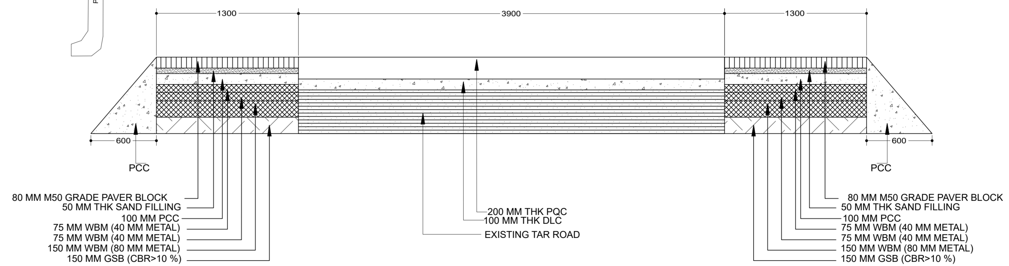
1:25 DETAILS OF INTERNAL ROAD (6.5 M WIDE) TO BE CONSTRUCTED ON EXISTING TAR ROAD
