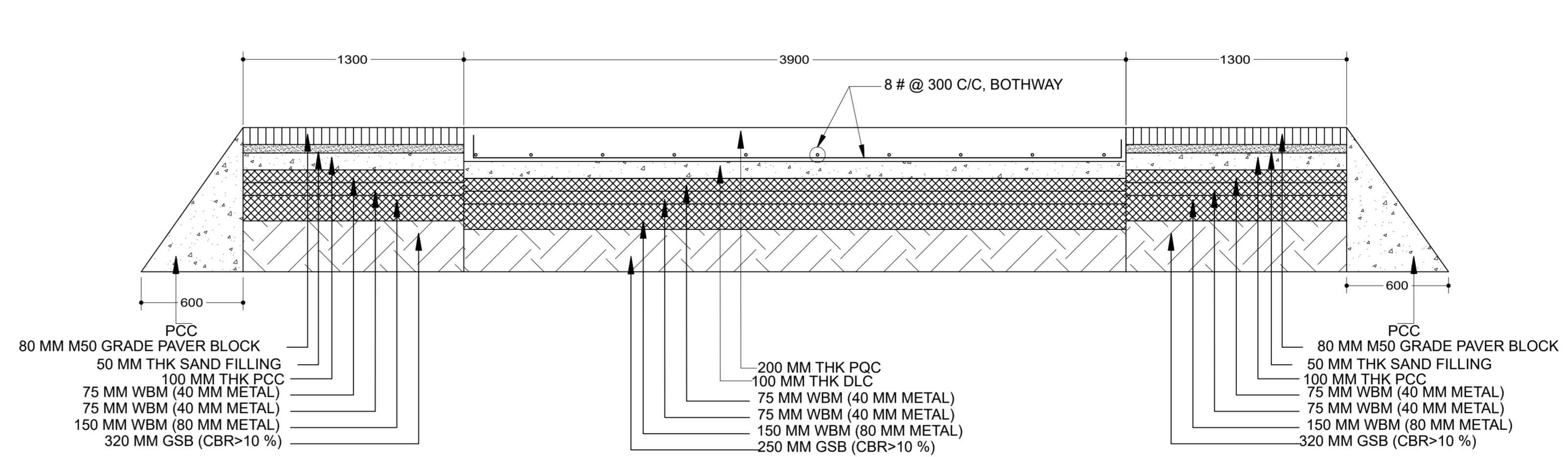
1:25 DETAILS OF INTERNAL ROAD (6.5 M WIDE)
